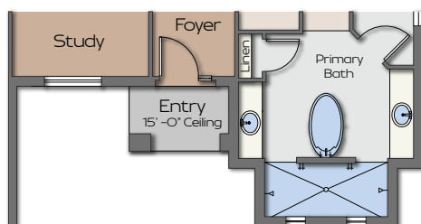
Coastal Elevation (38 Sq. Ft. Entry)
