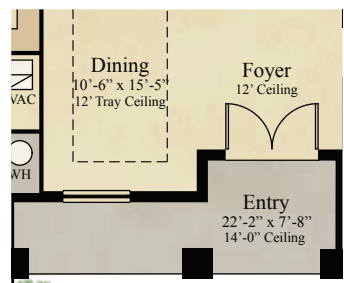
ELEVATION B 130 Sq. Ft. Entry
